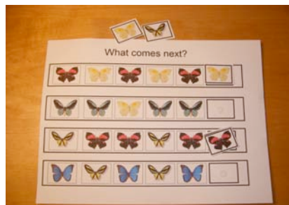
Butterfly pattern
